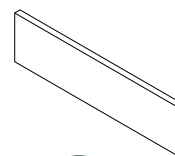
12 x2 457x118x15mm
