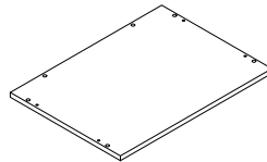
7 x1 550x400x18mm
