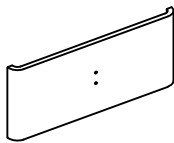
9 x2 500x218x30mm
